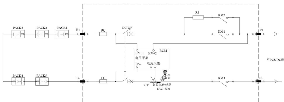
Figure 3.2.1-1 Schematic diagram of cluster control box
