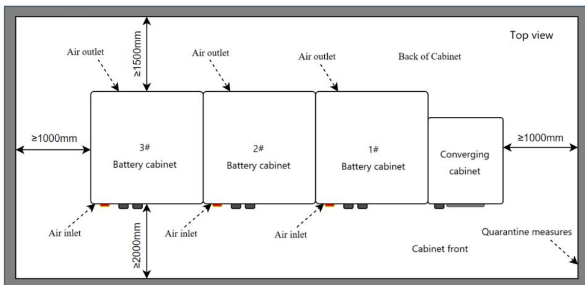
Figure 2.3.2-1 Space diagram
